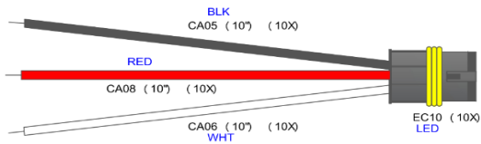
LED PIGTAIL TR5625
