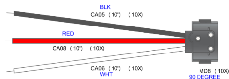
PL3 90 DEGREE 3 WIRE TR5624
