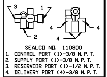
SPRING BRAKE CONTROL VALVE
