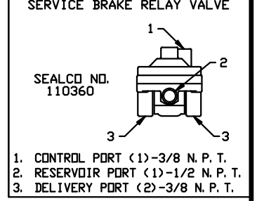
SERVICE BRAKE RELAY VALVE
