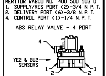
SERVICE BRAKE RELAY VALVE
