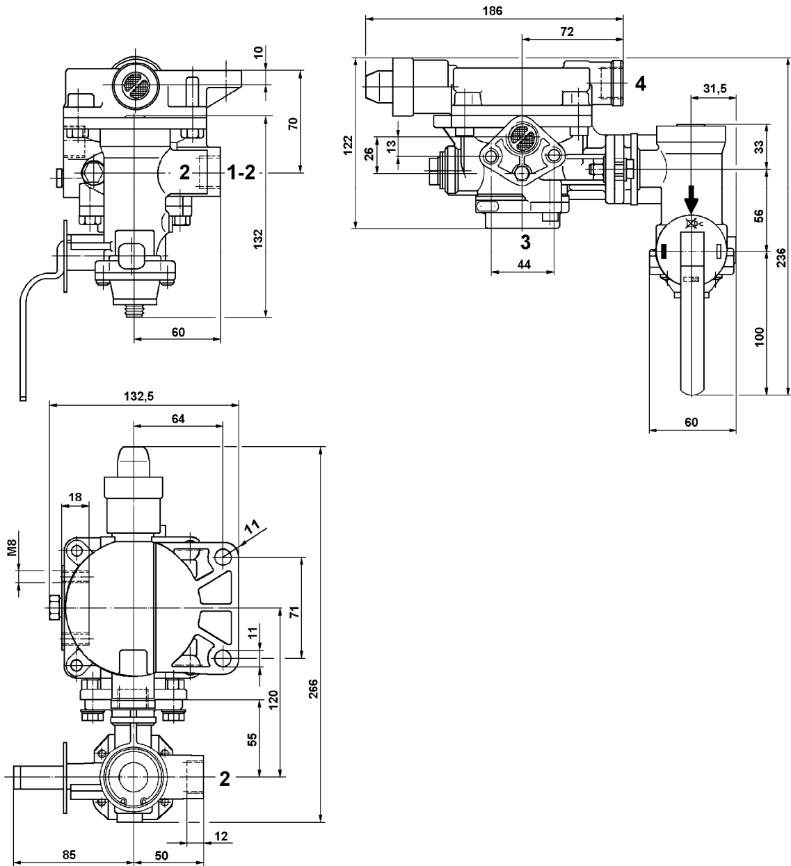
971 002 570 0: Combination trailer brake valve 971 002 150 0 with load sensing valve 475 604 011 0
