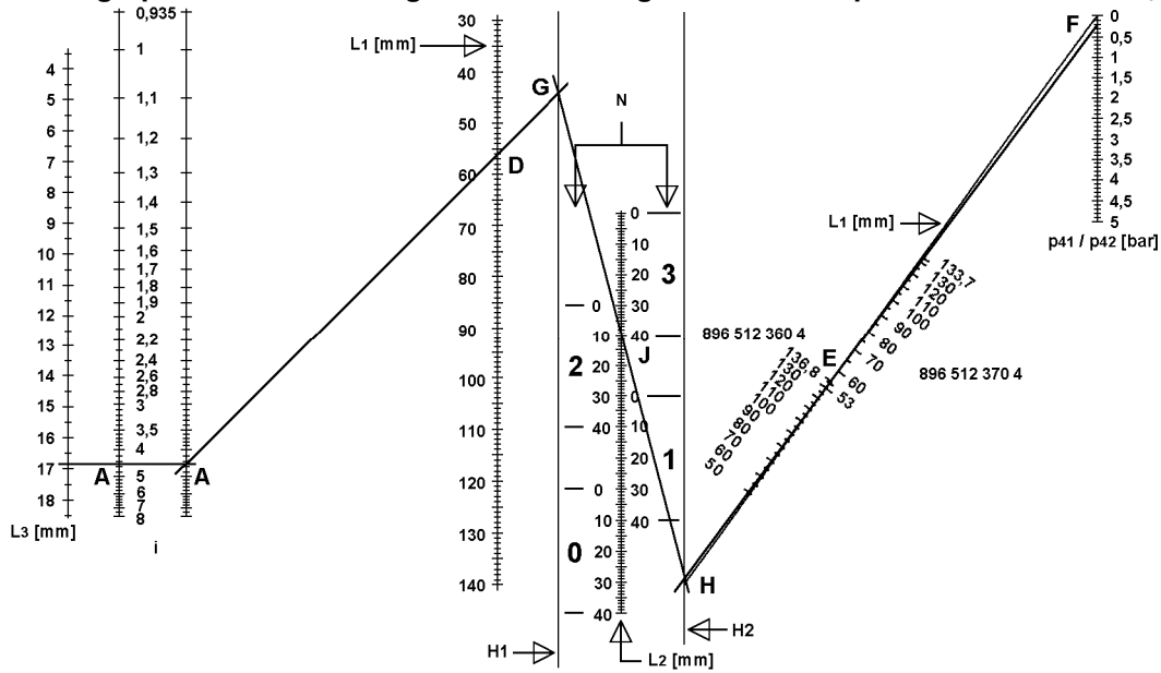
Nomograph II for determining the bolt set length L_2 and the spacers N as well as L_3
